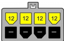
Stecker male
