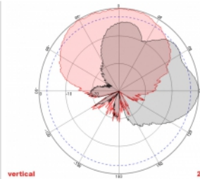
vertical 2400MHz
